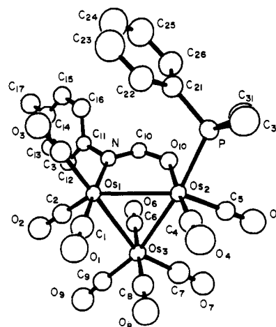
Figure 2. ORTEP diagram of (\mu\text{-H})(\mu\text{-}p\text{-CH}_3\text{C}_6\text{H}_4\text{NCHO})\text{Os}_3(\text{CO})_9[\text{P}(\text{CH}_3)_2\text{C}_6\text{H}_5] (V) showing 50% probability ellipsoids.
